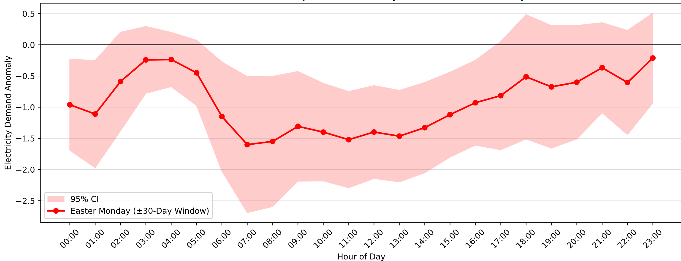
Gateshead Demand Anomaly: Easter Monday (2004–2017, \pm 30 -Day Window)
